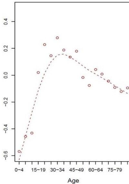
Male mortality profile
