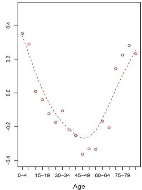
Female mortality profile
